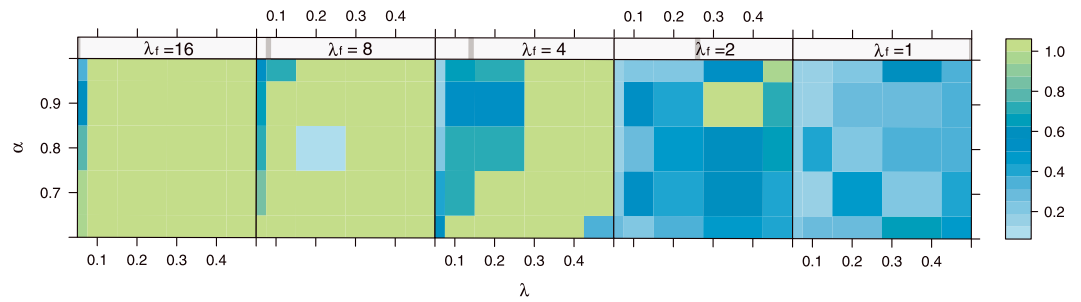
Figure 6. Variation in maximum tree fraction (%) as a function of precipitation intensity ( \alpha ), precipitation frequency ( \lambda ), and fire frequency ( \lambda_f ).
