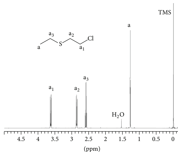
FIGURE 7: 1 H NMR spectrum of 2-CEES in CDCl 3 .
