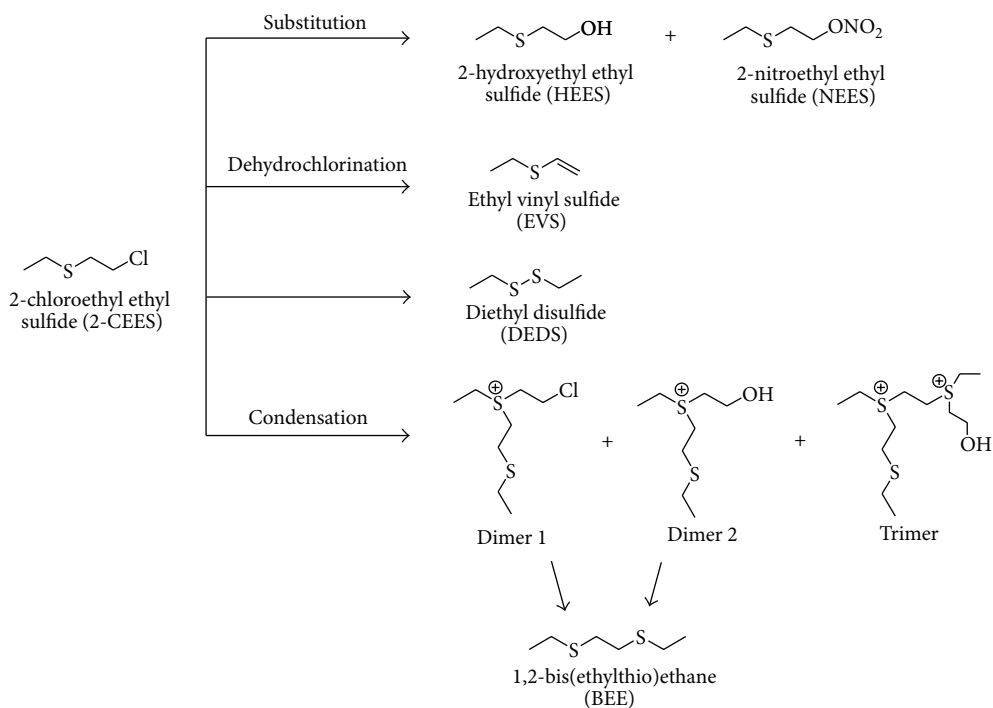
SCHEME 2: Degradation products of 2-CEES.
