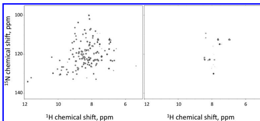
Figure 3. ^1\text{H} – ^{15}\text{N} HSQC spectra of N- \beta GRP (0.5 mM) in the absence (left) or presence (right) of laminarin (1 mM) at 25 °C and pH 6.5.
