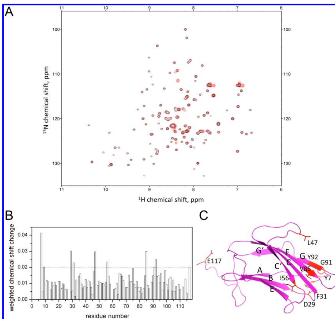
Figure 2. Mapping of the ligand binding site on P. interuptella N- \beta GRP by NMR titration of laminarihexaose at 25 °C and pH 6.5. (A) ^1\text{H} - ^{15}\text{N} HSQC spectra of N- \beta GRP (0.5 mM) in the absence (black) or presence (red) of laminarihexaose (3 mM). (B) Chemical shift changes undergone by the backbone ^{15}\text{N} - ^1\text{H} groups. The weighted average of chemical shift changes of an ^{15}\text{N} - ^1\text{H} group was calculated by using the formula \{[\Delta\text{H}^2 + (\Delta\text{N}/5)^2]/2\}^{1/2} , where \Delta\text{H} and \Delta\text{N} represent ^1\text{H} and ^{15}\text{N} chemical shift changes, respectively. (C) Residues undergoing a chemical shift perturbation of >0.02 ppm upon laminarihexaose titration are colored red.
