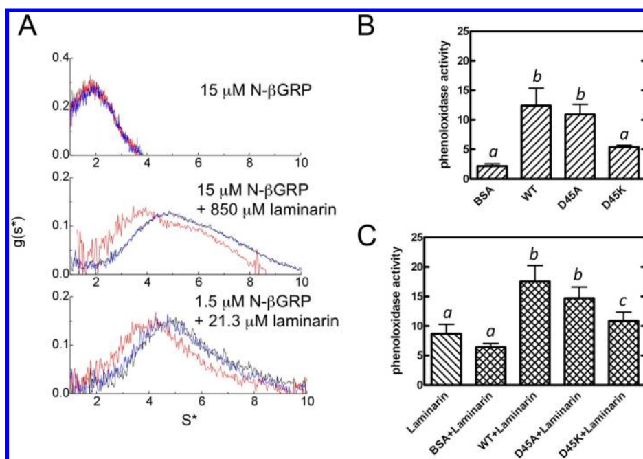
Figure 8. Electrostatic interactions play a role in the formation of the N- \beta GRP- \beta -1,3-glucan macro complex. (A) Sedimentation velocity profiles for N- \beta GRP (wide type, black; D45A, blue; and D45K, red) in the presence of laminarin. (B and C) Activation of the prophenoloxidase pathway by N- \beta GRP and mutants without (B) or with laminarin (C). Samples of plasma ( S \mu\text{L} ) were mixed with protein alone or with protein and laminarin. After incubation at room temperature for 15 min, phenoloxidase activity was measured using dopamine hydrochloride as a substrate, as described in Materials and Methods. The bars represent the means \pm the standard error of data from three sets of measurements on a pooled plasma sample. Bars labeled with different letters ( a , b , and c ) are significantly different [analysis of variance (ANOVA); p < 0.05 ].
