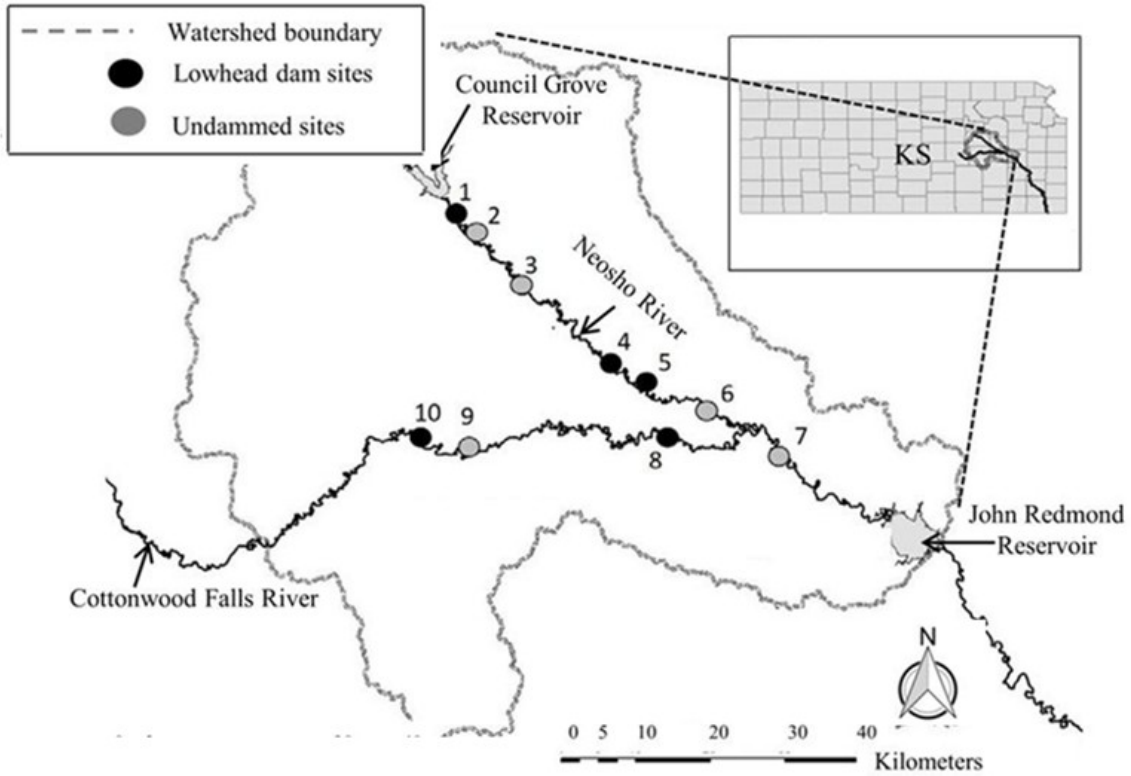
Figure 3.2. Map of study area representing ten sampling sites located along the Neosho and Cottonwood Rivers, KS. Black dots represent low-head dam sites and gray dots undammed sections of the rivers.
