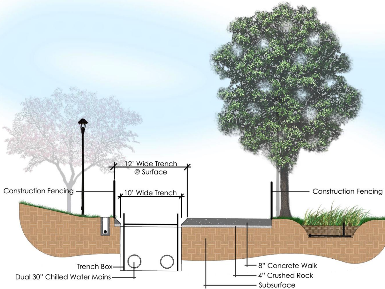
SECTION LOOKING NORTH DOWN MID CAMPUS DRIVE
