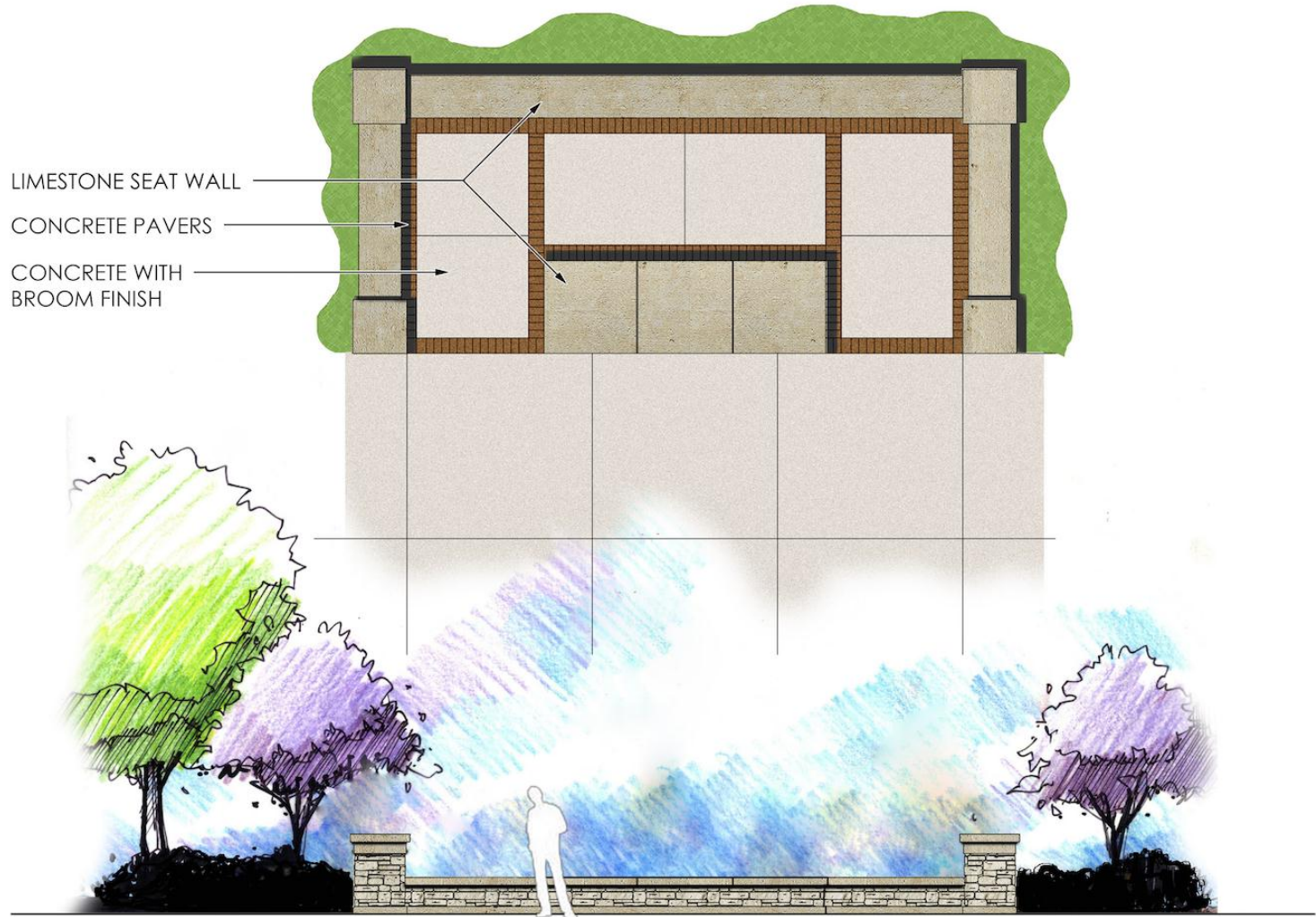
SEATING AREA ELEVATION & PLAN
